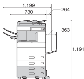
e-STUDIO2528A/3528A/4528A/5528A 寸法図 (mm)
