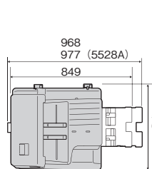
e-STUDIO2528A/3528A/4528A/5528A 寸法図 (mm)
